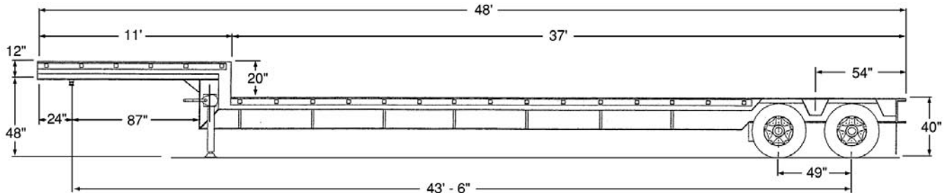
TANDEM AXLE MODEL SHOWN
