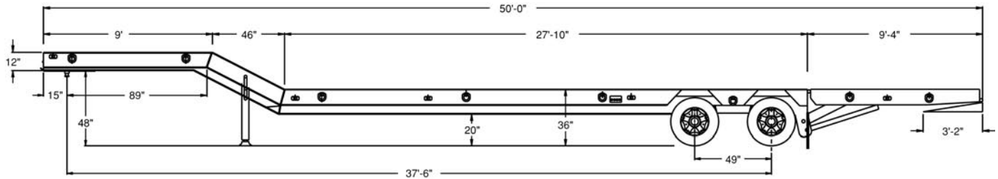
STANDARD 30 DEGREE GOOSENECK MODEL SHOWN
