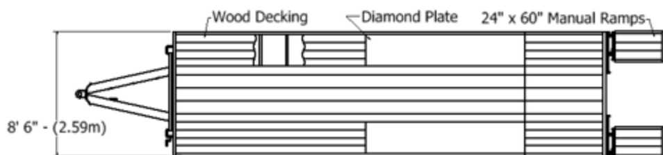
Standard Trailer Dimensions
