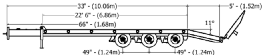
Standard Trailer Dimensions
