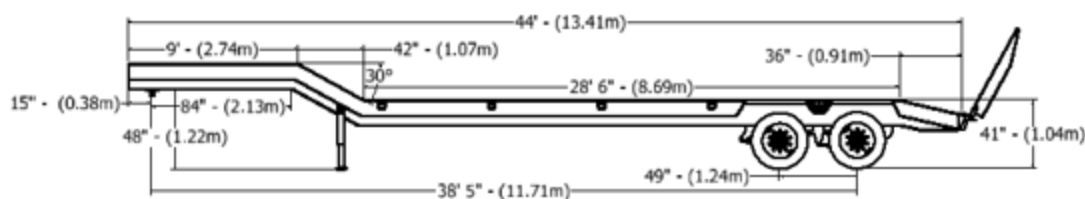
Standard Trailer Dimensions
