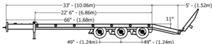
Standard Trailer Dimensions
