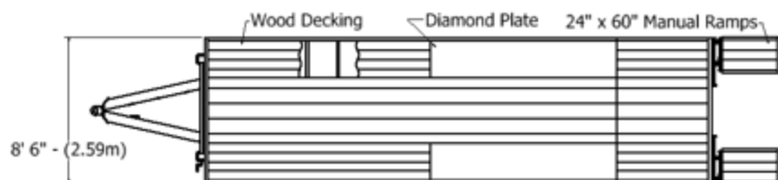
Standard Trailer Dimensions
