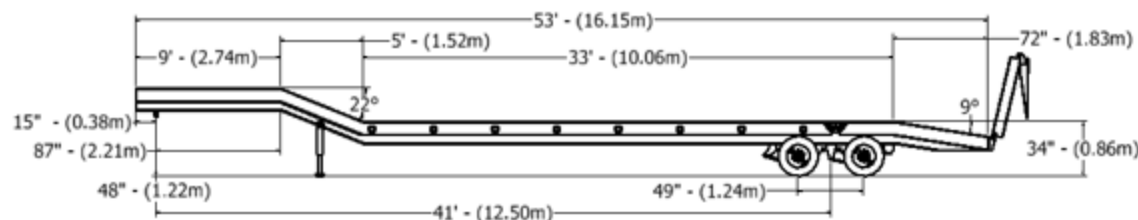
Standard Trailer Dimensions
