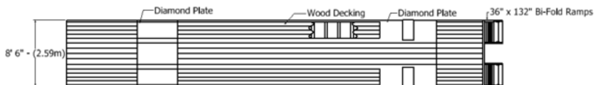
Standard Trailer Dimensions
