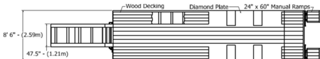
Standard Trailer Dimensions
