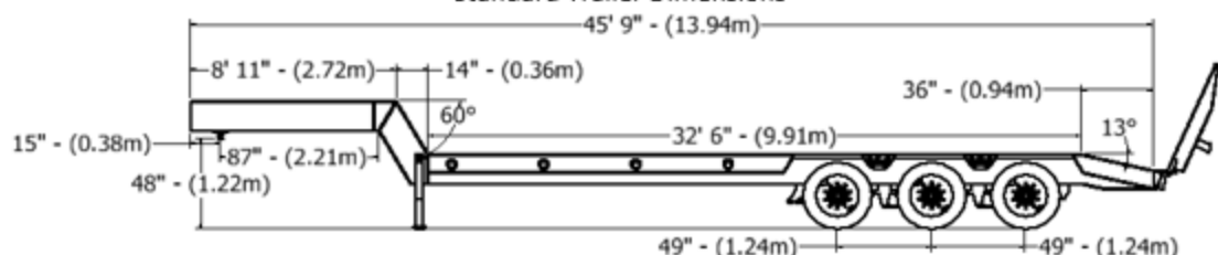
Standard Trailer Dimensions
